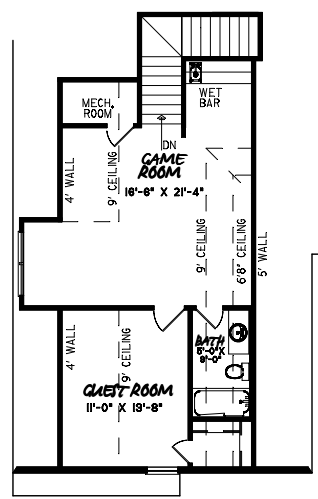
Upper Floor
